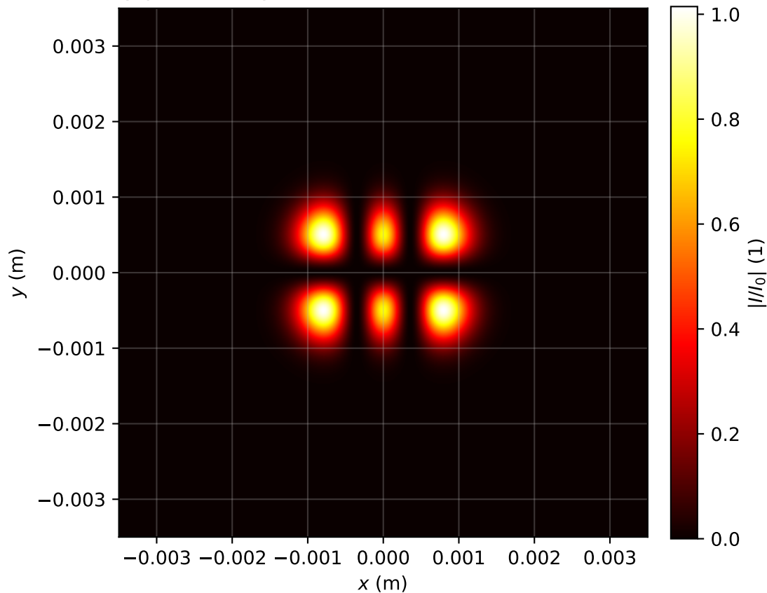
Intensity profile I(x, y, z = 0.318)/I_0 , P_{in}=0.5P_{cr} , artificial time
